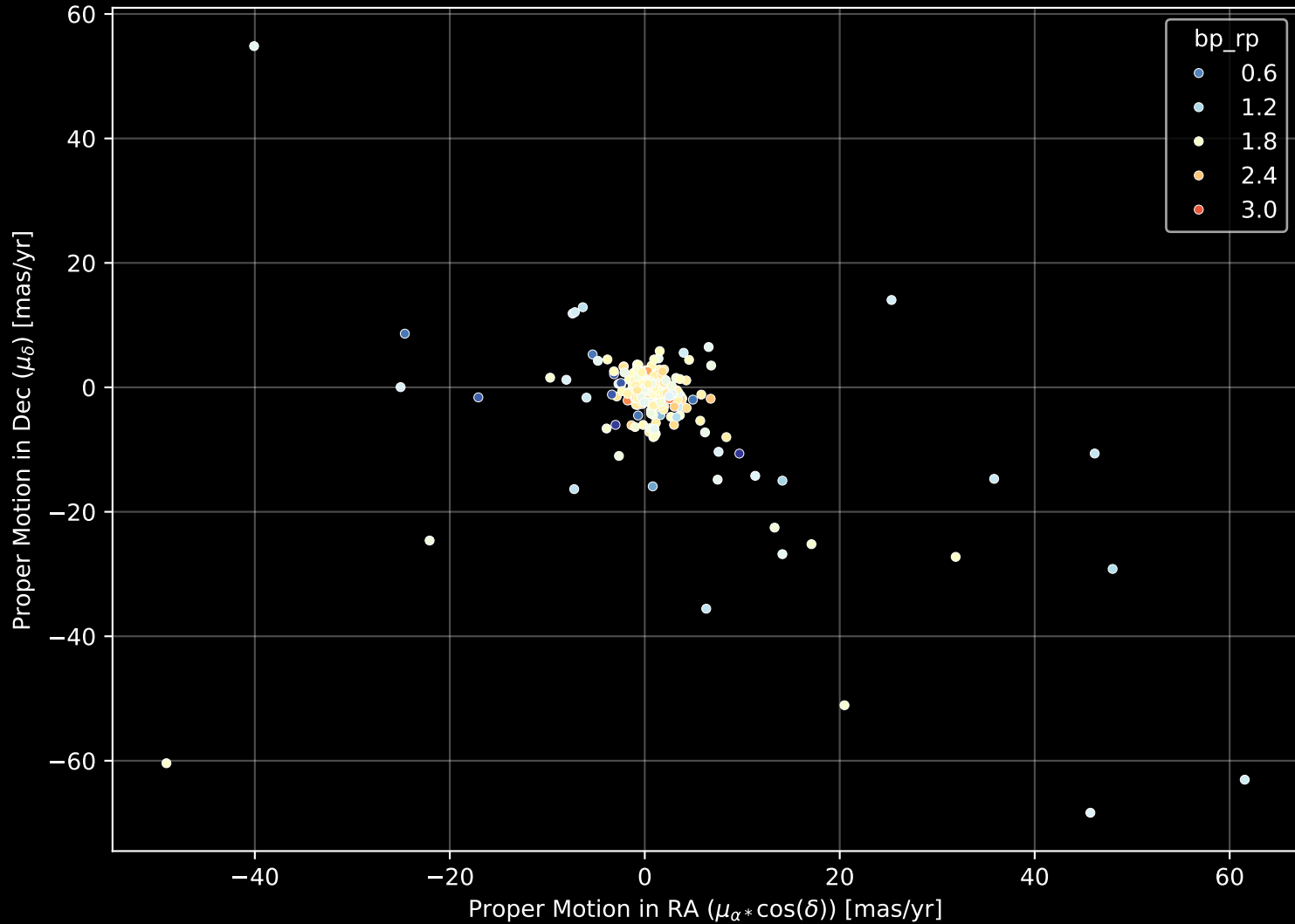
APOGEE DR17 Field: [140+12] Proper Motion Diagram (n= 352)
