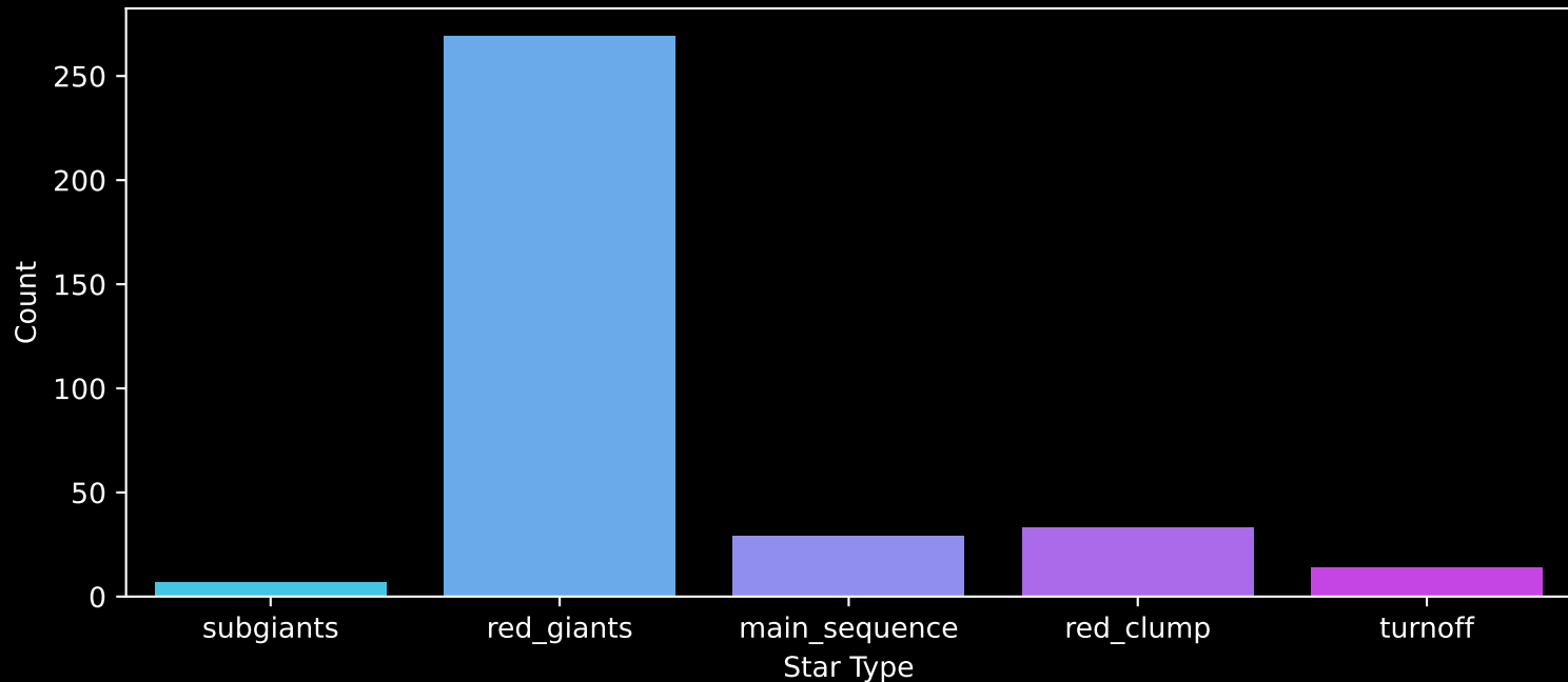
APOGEE DR17 Field: [140+12] Count plot of Star Type
