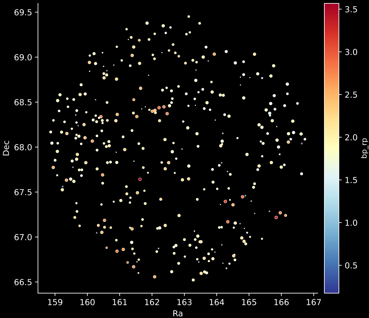
APOGEE DR17 Field: [140+12] Stars: 352
