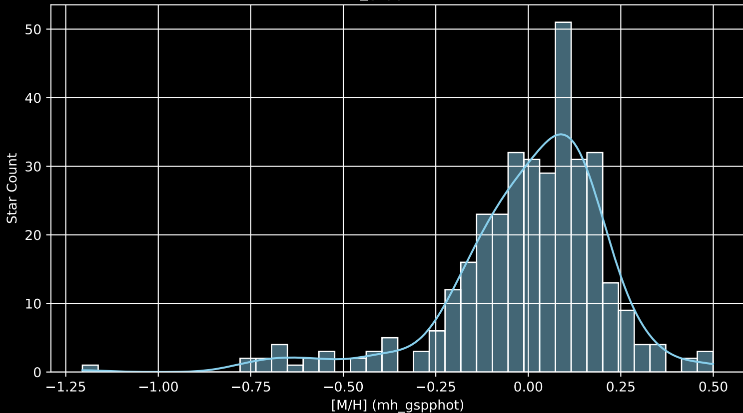
APOGEE DR17 Field: [140+12 [M/H] (mh_gspphot) (n= 349)
