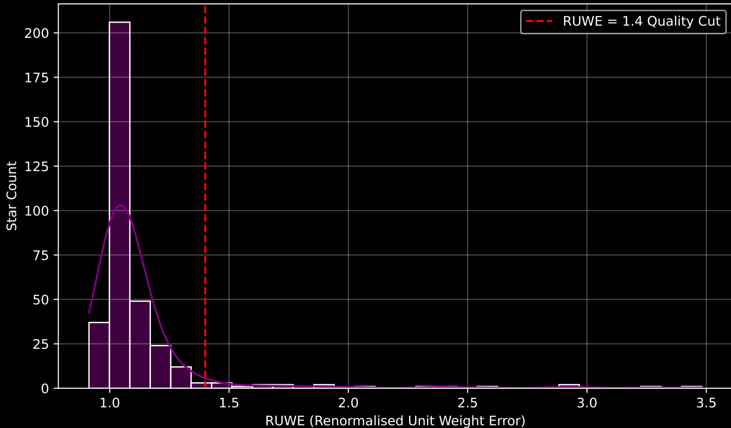
GAPOGEE DR17 Field [140+12] RUWE Distribution (n= 349)
