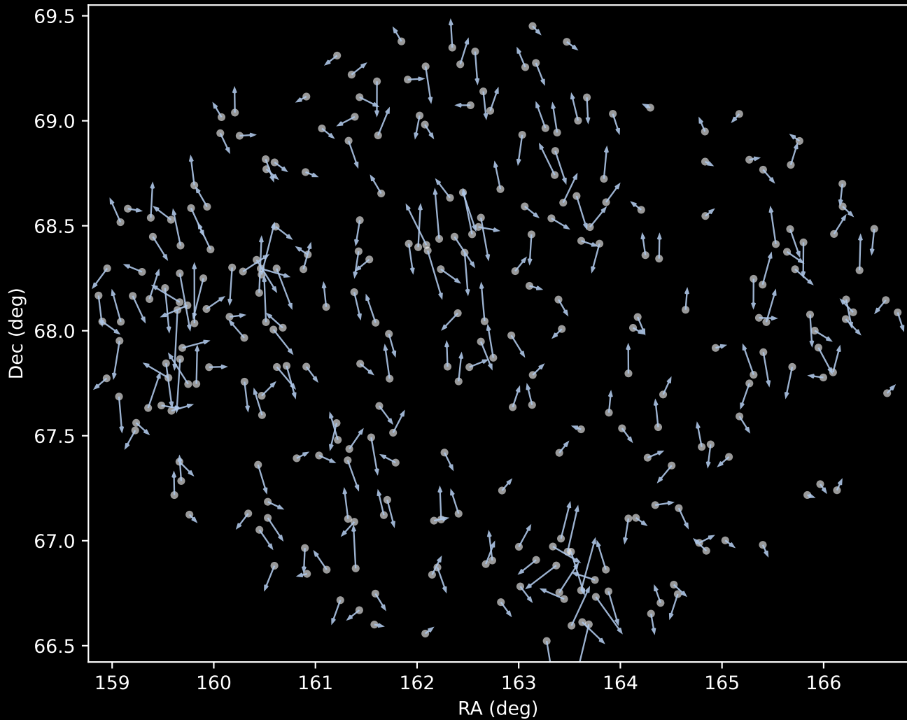
APOGEE DR17 Cluster 1 Proper Motion Vectors (n=285)
