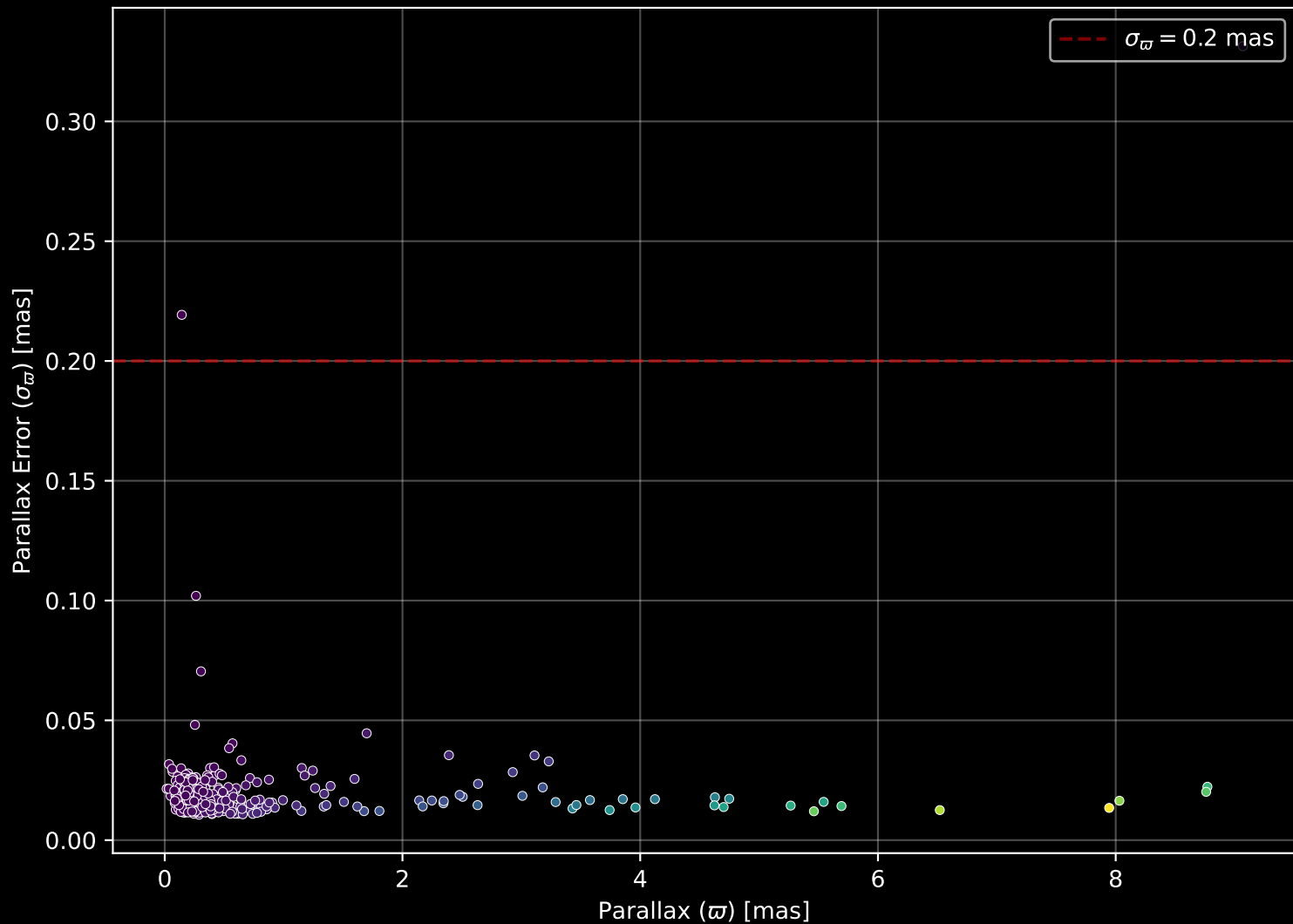
APOGEE DR17 Field: [140+12] Parallax Quality (n= 352)
